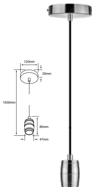
60SOCK113MVE27S ■ Satin
