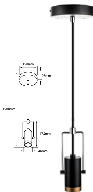
60SOCK114MVE27N ■ Negro/Bronce
